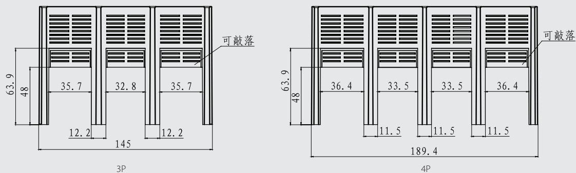
MDM5-400 端子罩
