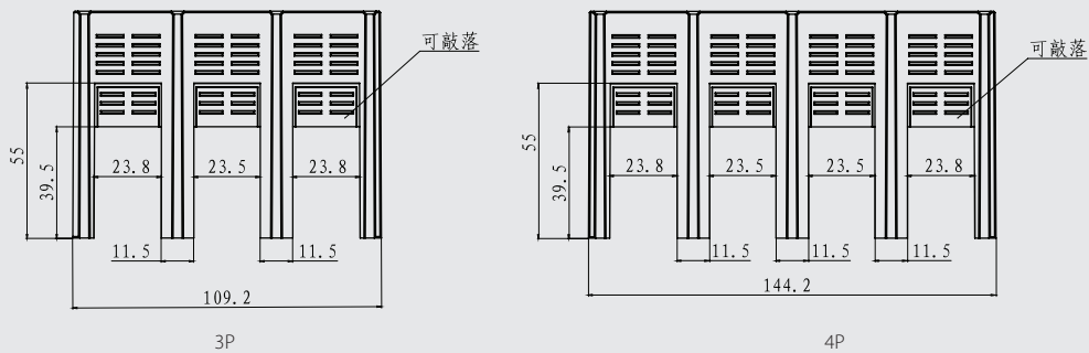
MDM5-250 端子罩
