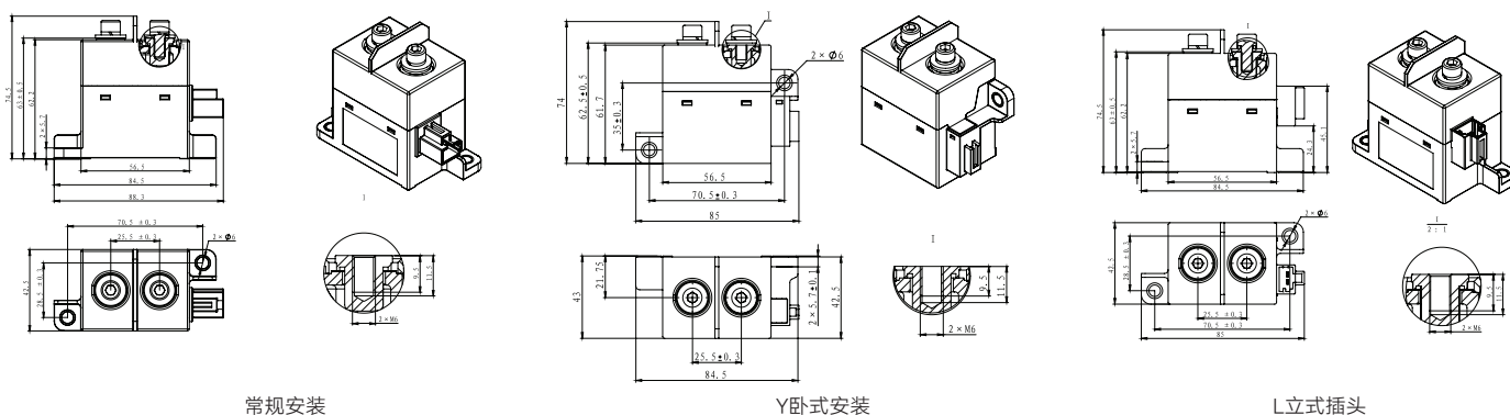
NDZ3AT-300C
