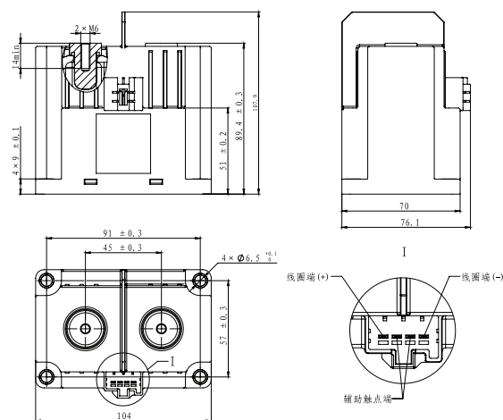
NDZ3AT-25010H
