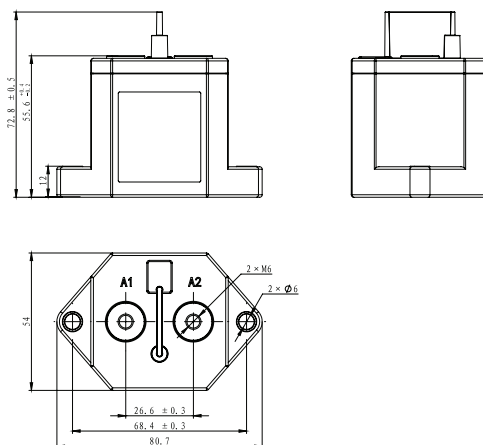
NDZ3AT-300R
