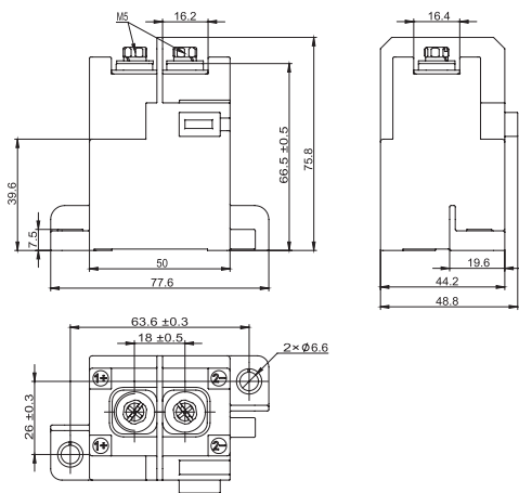
NDZ3T-100
