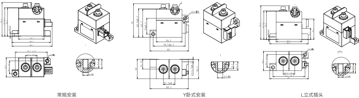
NDZ3AT-250C
