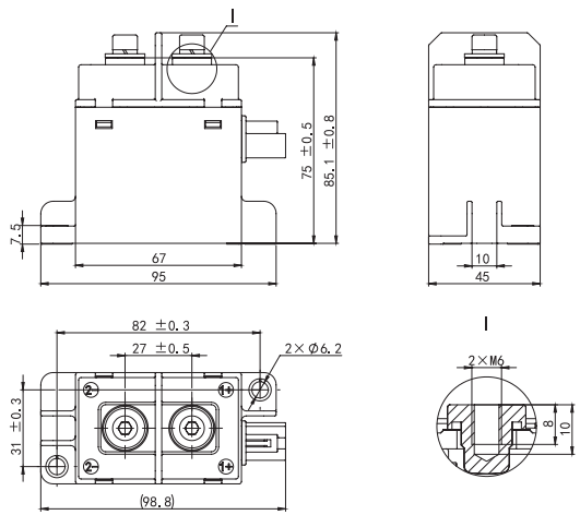
NDZ3AT-200
