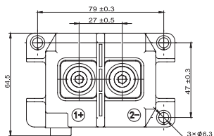
NDZ3T-400
