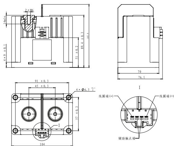
NDZ3AT-35010H
