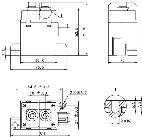
NDZ3AT-150B
