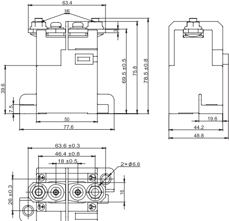
NDZ3T-100P
