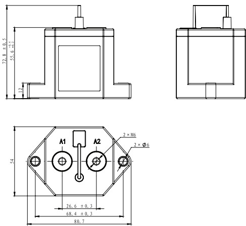
NDZ3AT-150R
