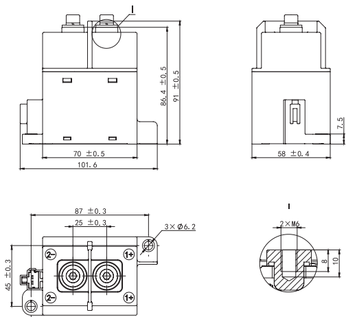
NDZ3AT-400
