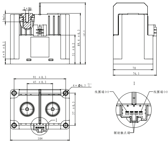
NDZ3AT-50010H
