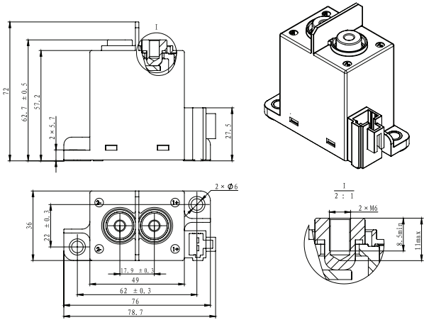
NDZ3AT-200G
