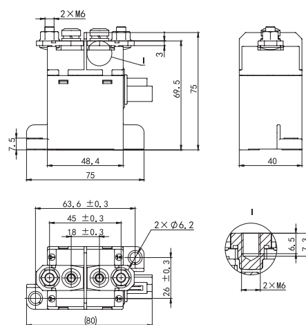
NDZ3AT-150CP
