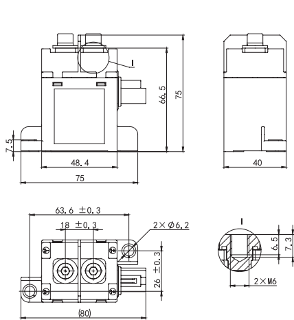
NDZ3AT-120
