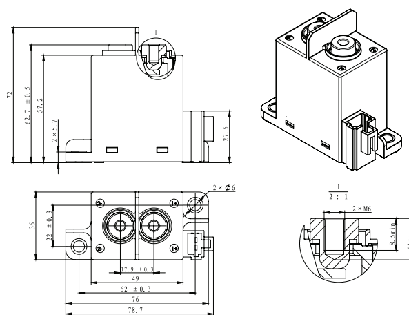
NDZ3AT-150G
