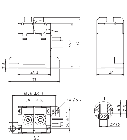
NDZ3AT-150C
