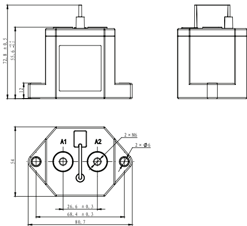
NDZ3AT-350R
