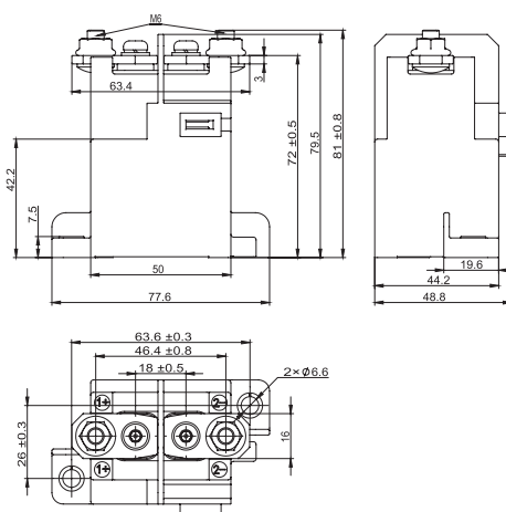
NDZ3T-150P
