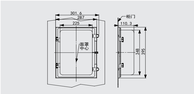
b. NDW1A-2000/3200/4000/6300产品的IP54透明罩外形尺寸
